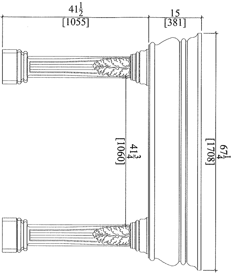
FRONT VIEW
