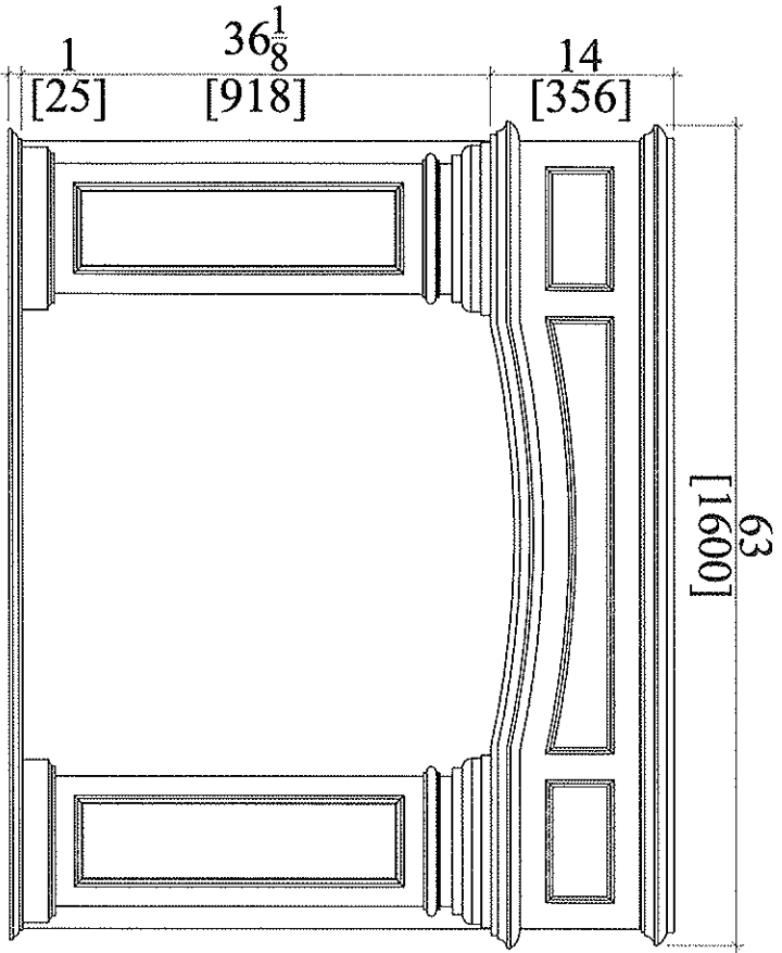
FRONT VIEW
